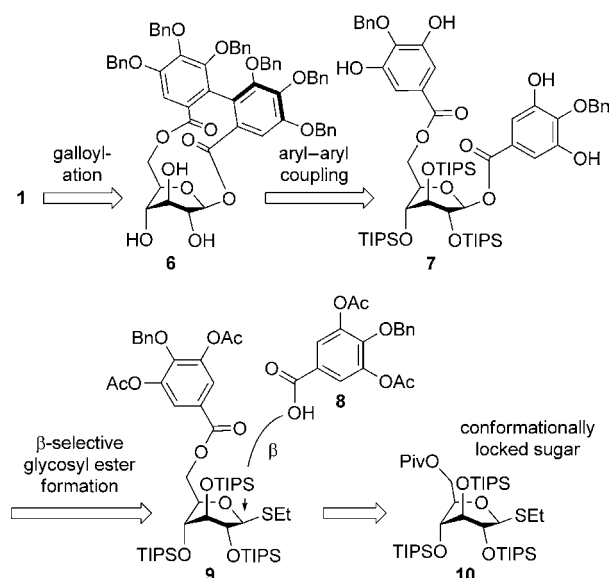
Scheme 2. Retrosynthetic analysis of daidivin ( 1 ).
